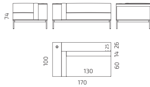
Module B left handed configuration S126-2CLB
